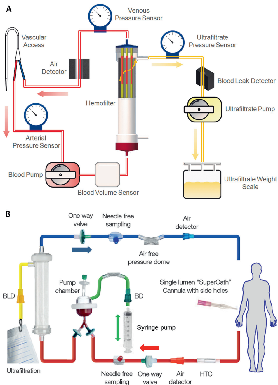
FIGURE 1 UF Circuit
