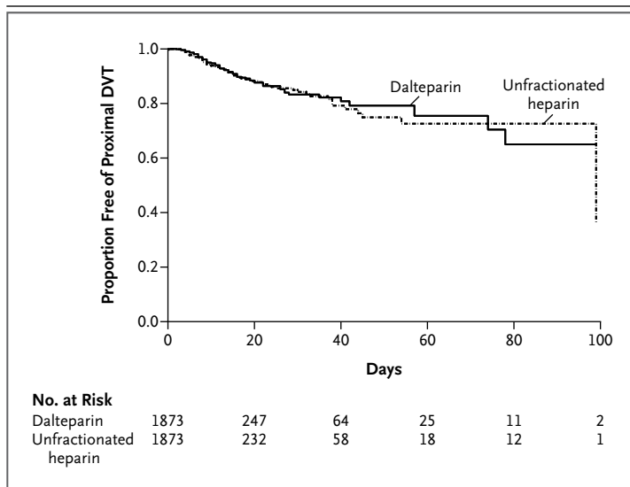
Figure 1. Kaplan–Meier Curves for the Time to Proximal Deep-Vein Thrombosis.
