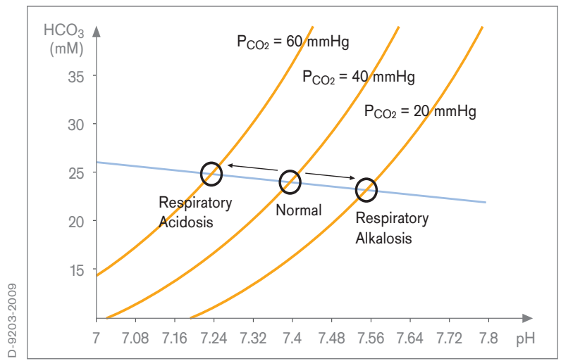
Davenport diagram
