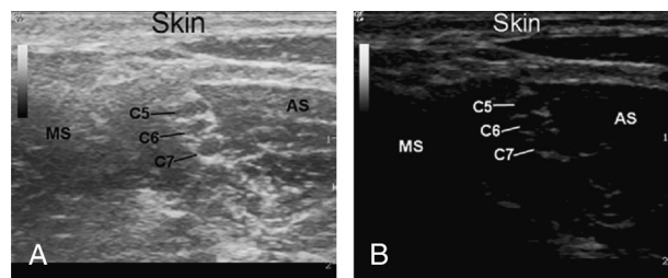
FIGURE 1. Incorrect overall gain settings. This is a short axis view of the brachial plexus. A, Overall gain set too high. B, Overall gain set too low. AS, anterior scalene muscle; C5, C6, C7, the fifth through seventh cervical nerve roots; MS, middle scalene muscle.
