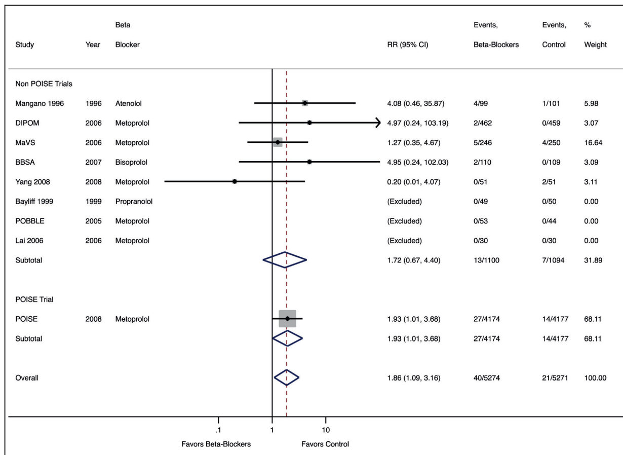
FIGURE 4 Effect of Perioperative Beta Blockade on In-Hospital or 30-Day Nonfatal Stroke in RCTs After Exclusion of the DECREASE Family of Trials, Within Subgroups Defined by the POISE-1 Trial Versus Other Trials
