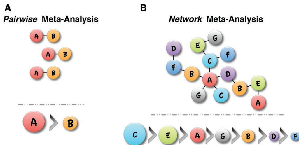
Fig. 1. A visual representation of two forms of meta-analysis. Each circled letter represents a distinct treatment, and each line represents a randomized controlled trial comparing two interventions. A traditional pairwise meta-analysis (A) compiles multiple trials comparing two treatments ( above dashed line ) and produces an estimate of the relative net benefits of the two ( below dashed line ). A network meta-analysis (B) uses a process allowing indirect comparisons of multiple, diverse treatments ( above dashed line )—relatively few of which have been directly compared—to provide an estimate of the relative net benefits of all included interventions ( below dashed line ).
