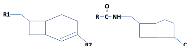
Fig. 2. Simplified structure of cephalosporin (left) with R1 and R2 side-chain location and penicillin (right). The square represents the β-lactam ring, and on the right the dihydrothiazine ring for cephalosporins and the thiazolidine ring for penicillins.
